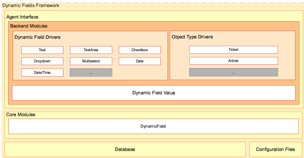
Figure 3.5: Dynamic Fields Framework
