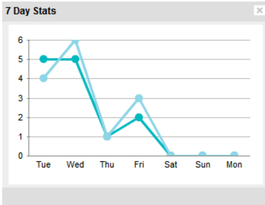
Figure 3.3: Dashboard Widget
