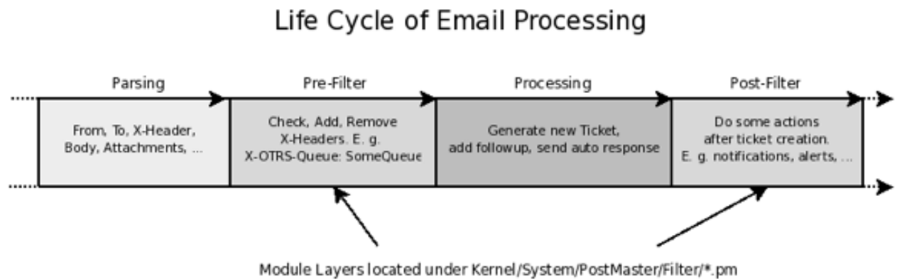
Figure 3.8: Email Processing Flow
