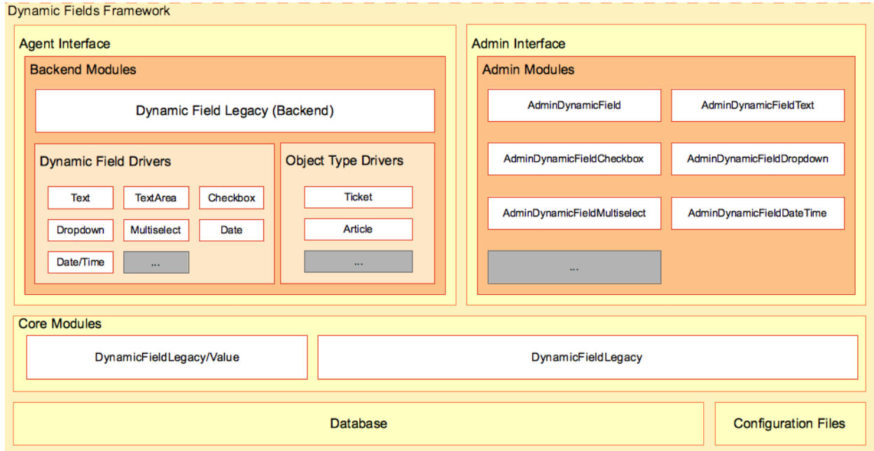
Figure 3.4: Dynamic Fields Framework
