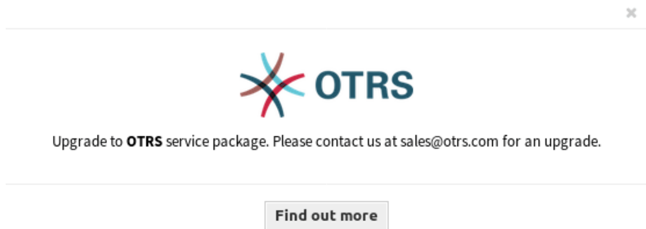
Fig. 5.8: Upgrade Dialog
