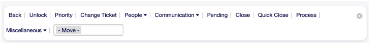
Fig. 6.38: Ticket Menu
