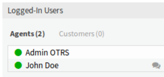
Fig. 8.2: Available Agents
