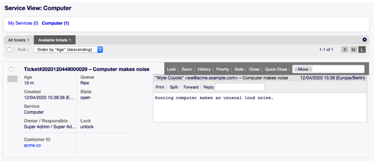
Fig. 6.14: Floating Menu of Large Service View
