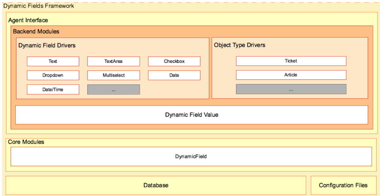
Fig. 5: Dynamic Fields Framework
